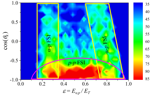
FIG. 7. Experimental joint energy-angular distributions in the Jacobi “Y” system for the E_T = 5.8 - 9 MeV bin.
