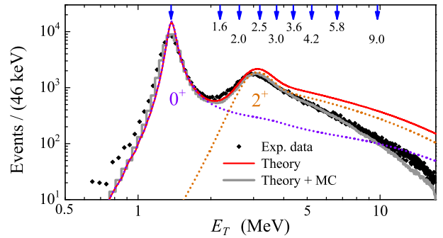
FIG. 2. Experimental invariant-mass spectrum of {}^6\text{Be} and the fitted theoretical result. Within this work the data points show experimental data, solid curve – the theoretical result, and gray histogram – the Monte Carlo simulation. The dotted curves show the contributions of 0^+ and 2^+ states to the theoretical spectrum. The arrows indicate the boundaries of the energy bins used in this work.
