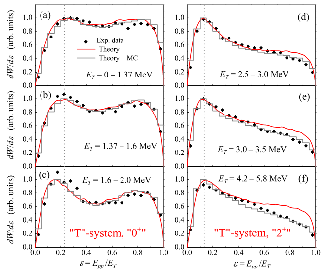
FIG. 4. Evolution of energy distribution in the Jacobi “T” system (between two-protons) with the decay energy. The left and right columns show the energy ranges where the 0^+ and 2^+ states dominant.
