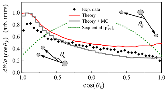
FIG. 6. Angular distribution in the Jacobi “Y” system for the E_T = 5.8 - 9 MeV bin.
